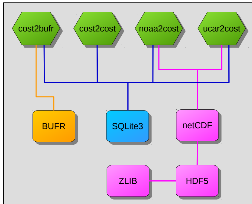
Illustration 1. GBGP application tools and their dependency packages
