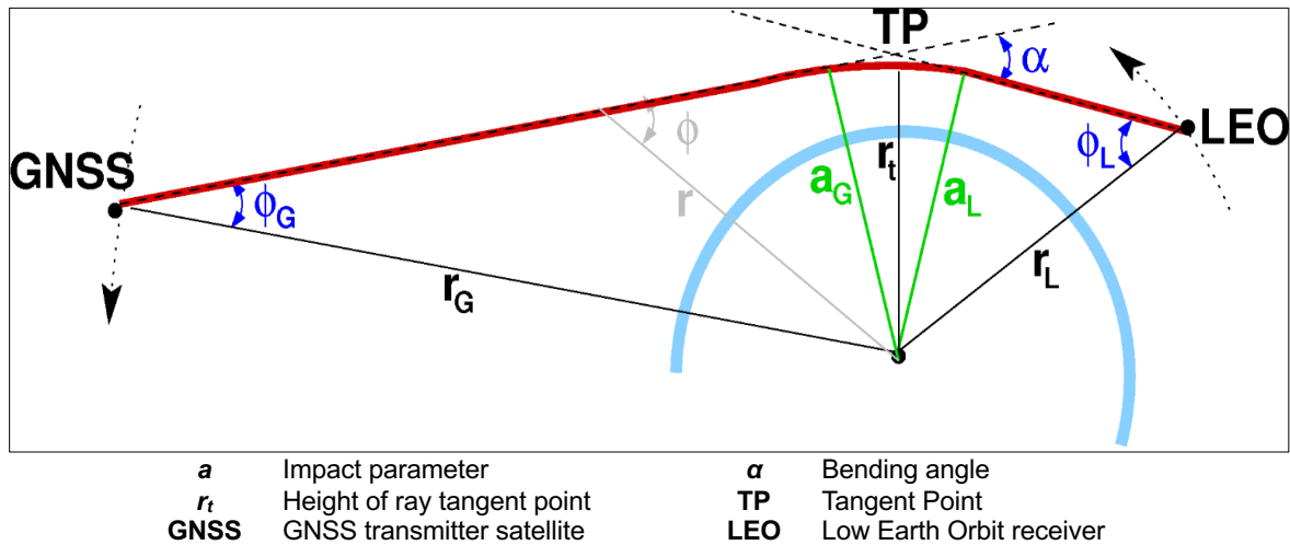
Figure 1. Schematic picture of the radio occultation geometry
